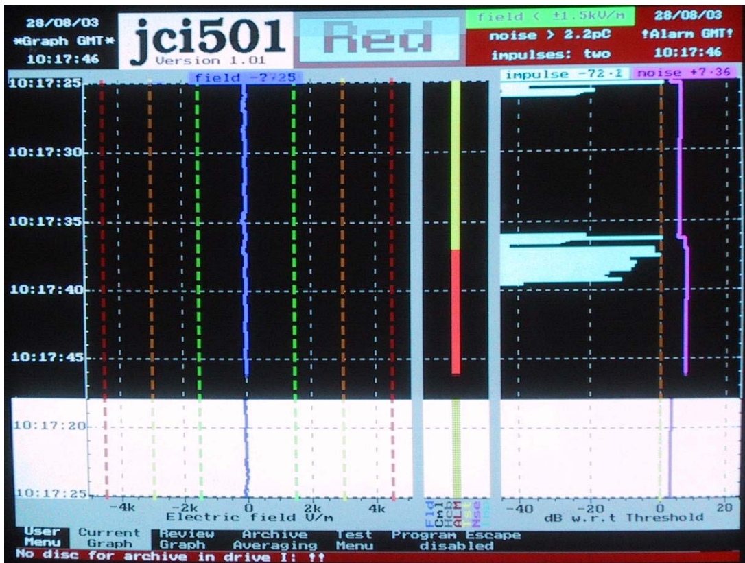
Normal operation showing Red alert due to high noise level and two impulses above impulse threshold within 100s. Electric field low.
