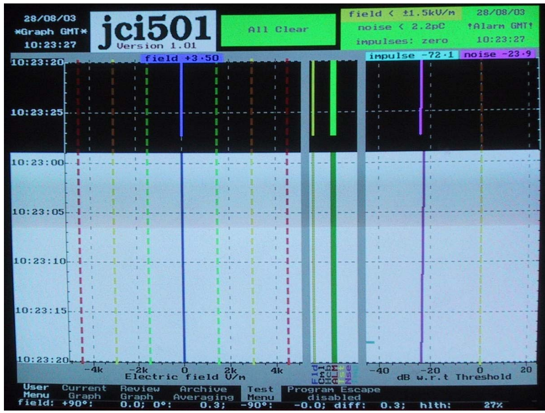
Operation with fieldmeter shielded and poor fieldmeter operational health indications
