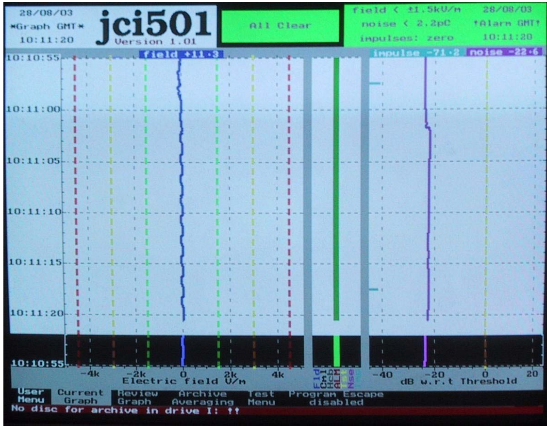
Normal operation – fieldmeter showing operational health testing signal
