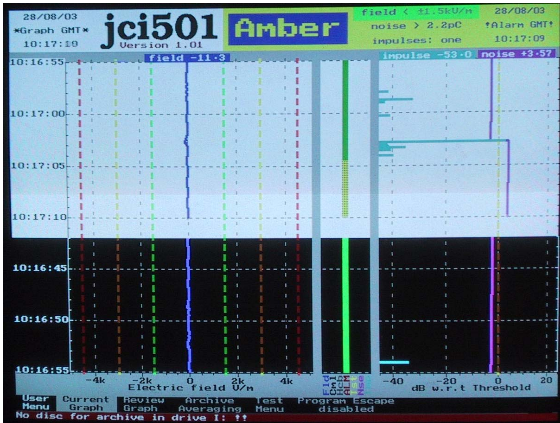
Normal operation showing response to impulse and noise signals going above threshold and giving 'amber' alert
