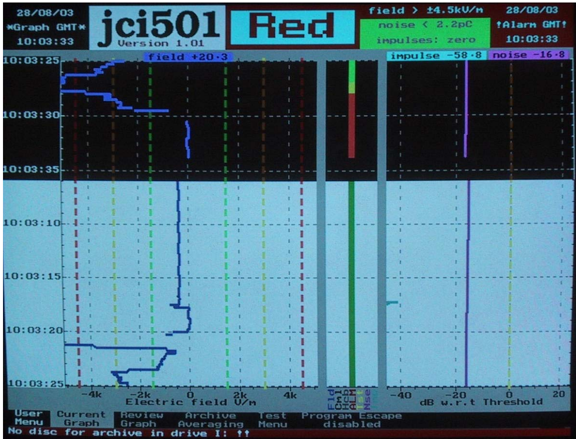
Excursion of electric field above red alert threshold level
